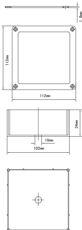
Hardware Fitting(optional) 预埋件尺寸图(选购)
